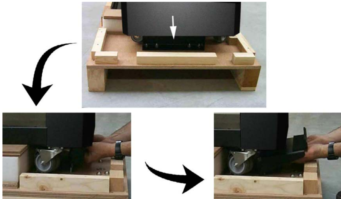
FIG 1-2 UNPACKING DC4SX STAGE 2
