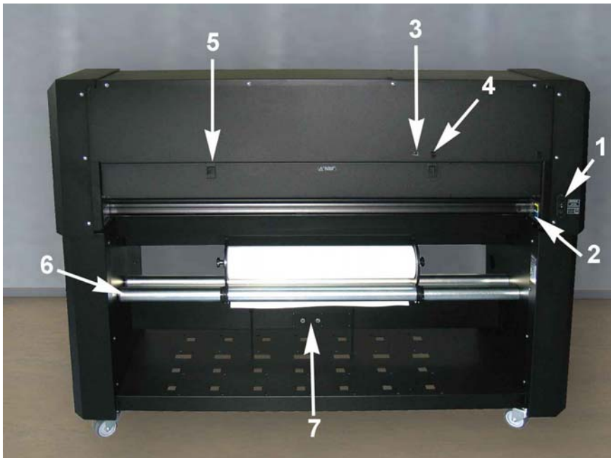
FIG 1-6 DC4SX, REAR VIEW
